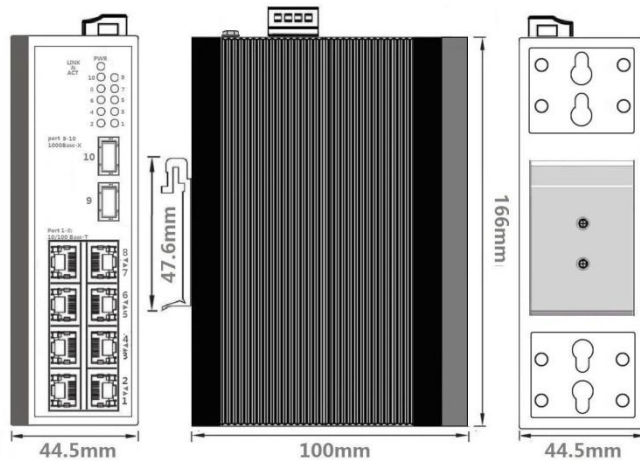
Din-Rail
