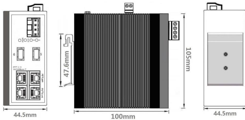
Din-Rail
