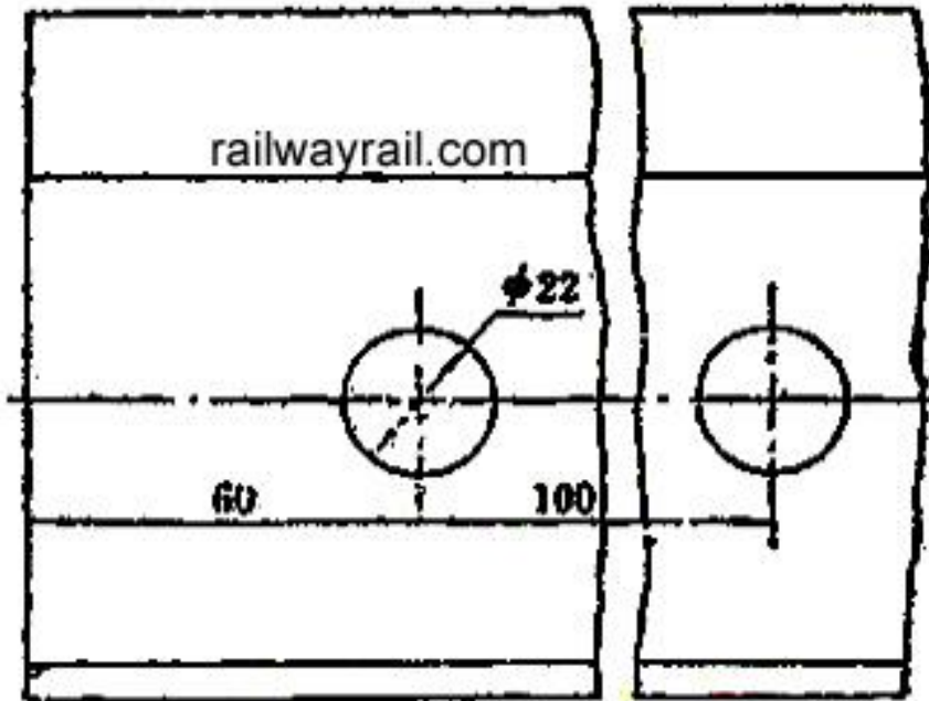
24kg/m Chinese steel rail (Size: mm)
